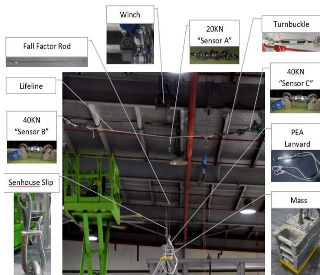
Figure 2: HLLS experimental set-up
